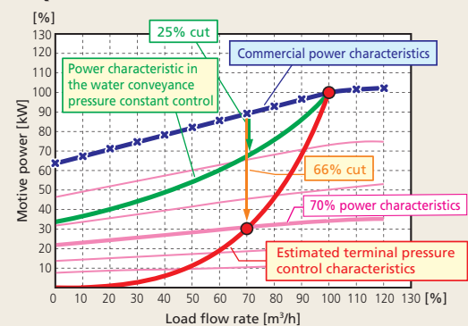
Q-P curve
